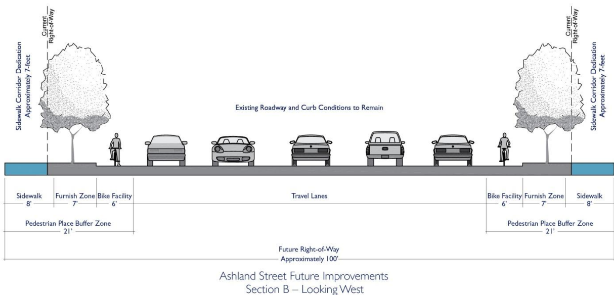
Exhibit 11-8 Ashland Street Cross Section
